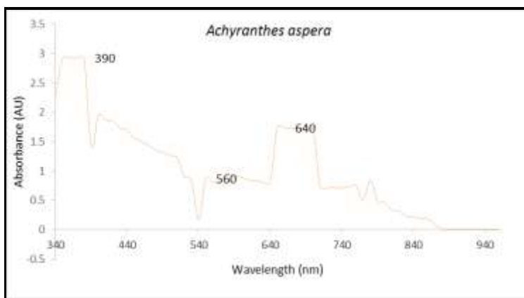
Fig.1: UV-Visible spectrum analysis of Achyranthes aspera L. leaves
